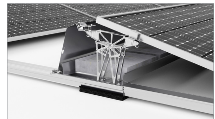
Ballasting Option
