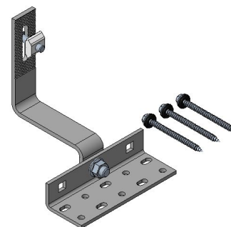
Adjustable Roof Hook TH05
